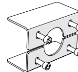
TAV5068 2x 6 mm 4x M16x65
